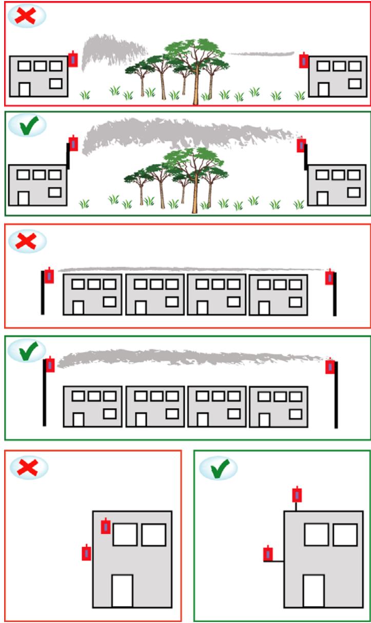
Figure. 1: Antenna Mounting
