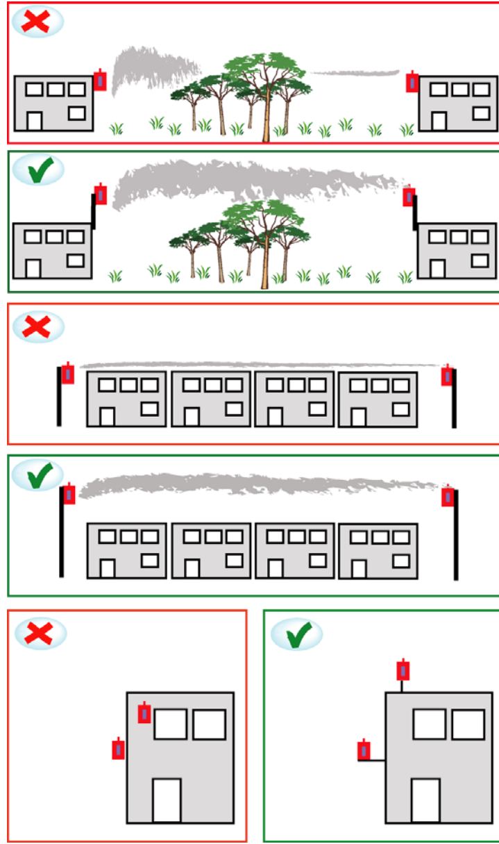
Figure. 1: Antenna Mounting
